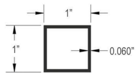
Industrial Grade Picket Cross Section
