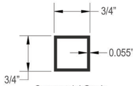
Commercial Grade Picket Cross Section
