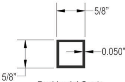
Residential Grade Picket Cross Section
