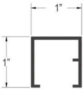
Residential Grade Rail Cross Section
