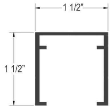
Industrial Grade Rail Cross Section
